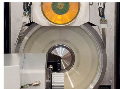
Agathon grinding machines equipped with PowerGrind technology
